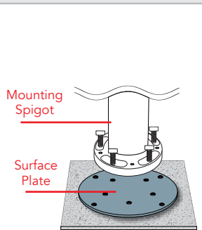
SURFACE PLATE
