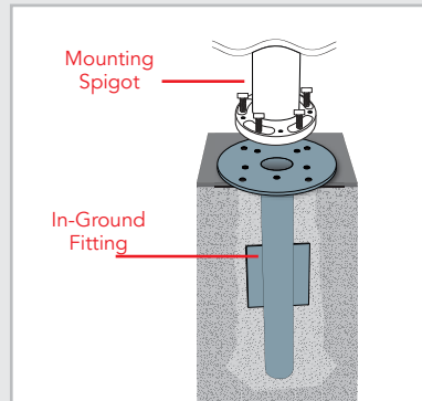
IN-GROUND ANCHOR
